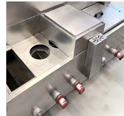
Two-tank system
